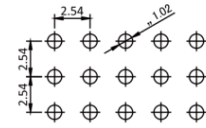
Recommended PCB Layout (PCB TOLERANCE ±0.05)
